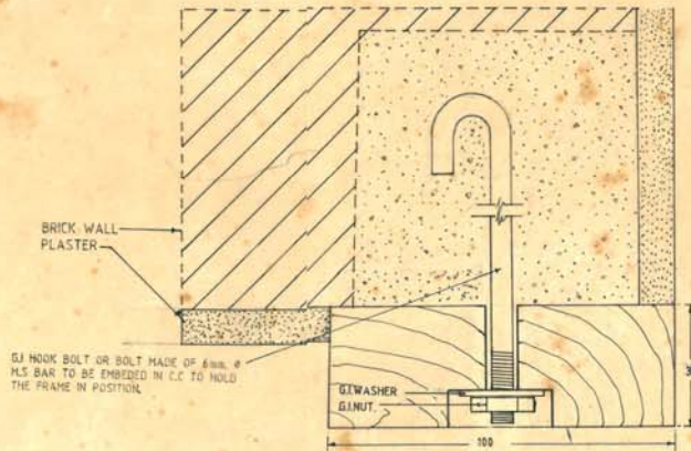
DETAIL OF FLAT FRAME FOR WARDROBE & ALMIRAH
