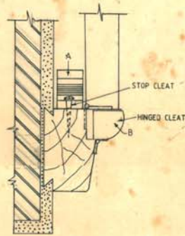
TYPICAL PLAN OF FRAME POSITION OF STOP CLEAT/HINGED CLEAT
