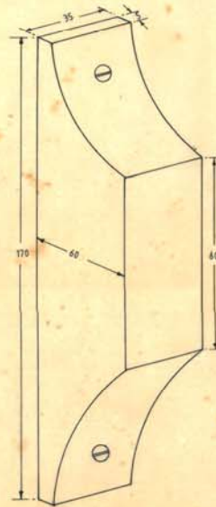
STOP CLEAT DETAIL AT-A
