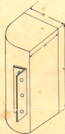
HINGED CLEAT DETAIL AT-B
