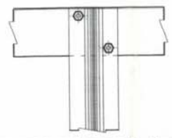
ELEVATION ( DETAIL AT 'B')
